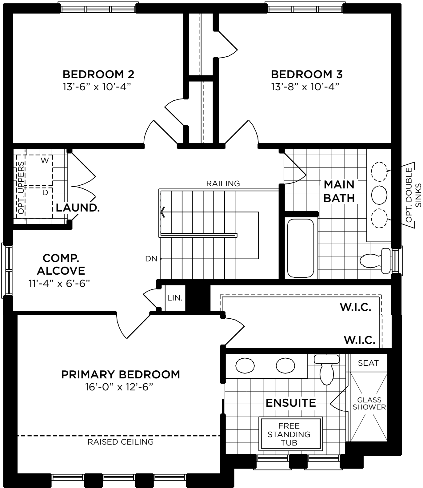
PART. SECOND FLOOR PLAN Elev. B
