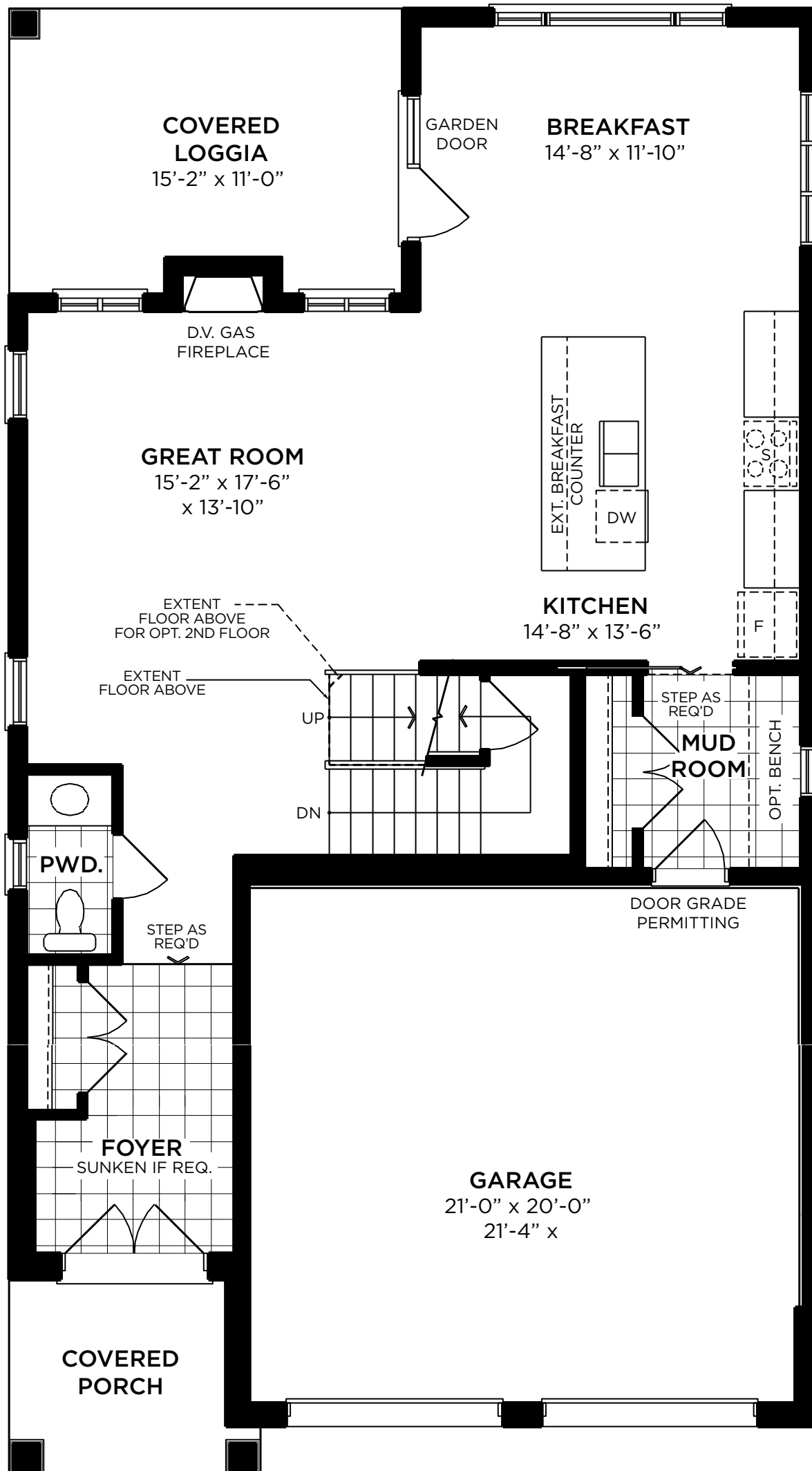
PART. GROUND FLOOR PLAN Elev. B & B2
