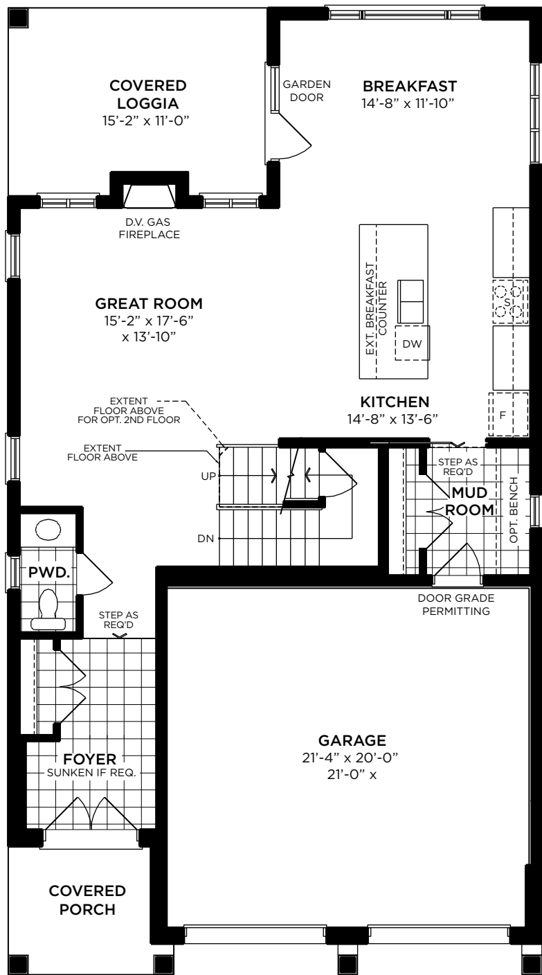
GROUND FLOOR PLAN Elev. A
